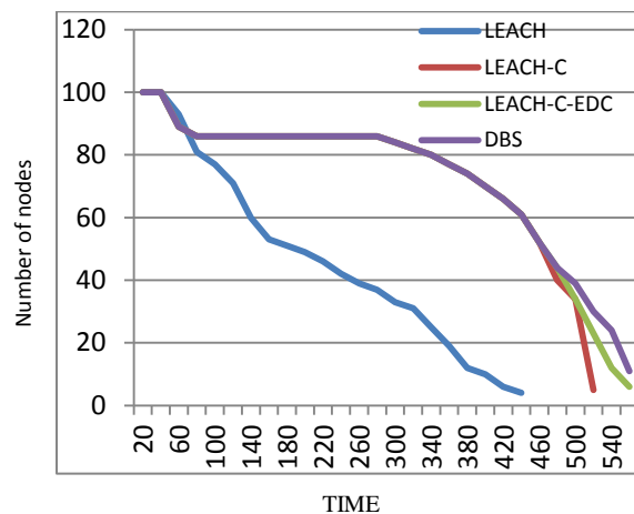
Figure 2. Number of alive nodes in each period
