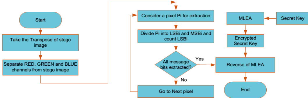
Fig. 4. Flowchart for extraction algorithm
