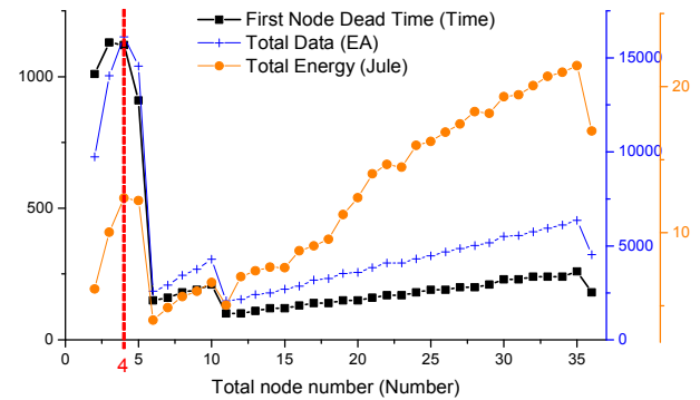
Figure 4: Result of network availability simulation
