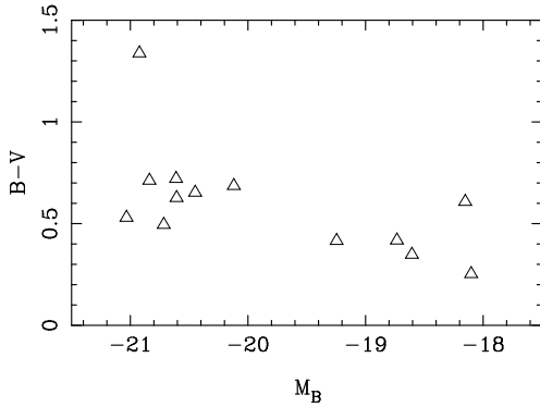
Figure 1. B - V color vs. absolute magnitude M_B diagram.
