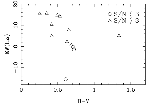
Figure 4. H\alpha equivalent width vs. B - V color diagram for the sample galaxies.
