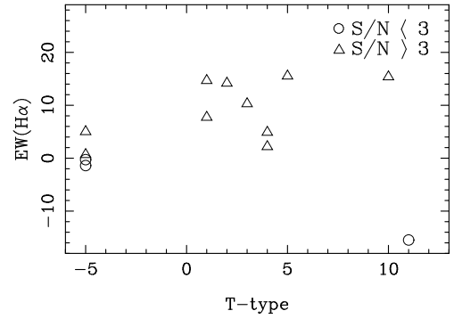
Figure 3. H\alpha equivalent width vs. T-type diagram for the sample galaxies.
