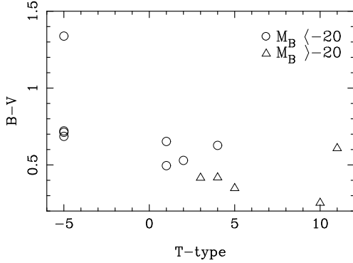
Figure 2. B - V color vs. T-type diagram, separated by M_B \sim -20 mag.
