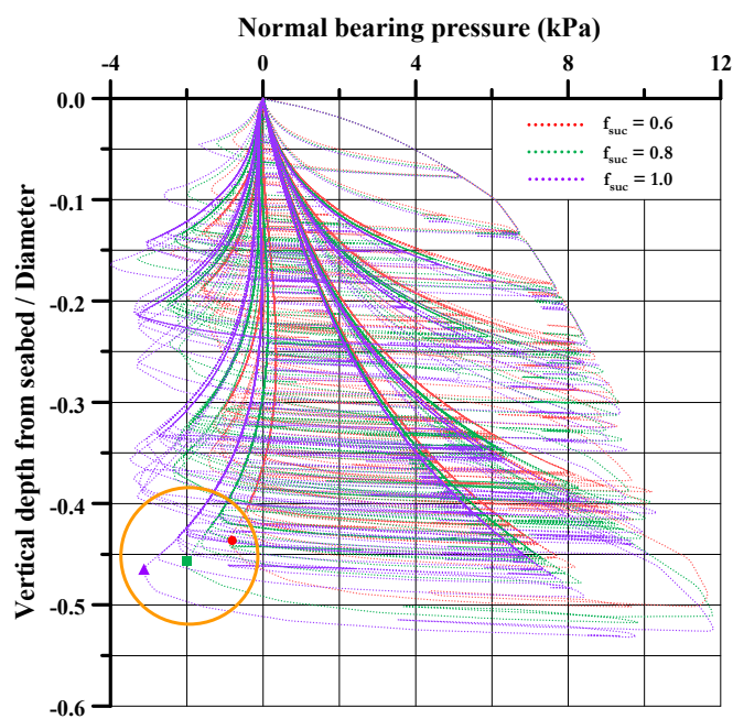
Fig. 11 Pipe embedment by suction resistance ratio variation.
