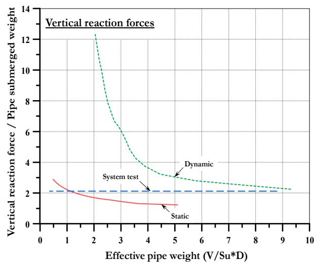
(b) Effective pipe weight effects.
