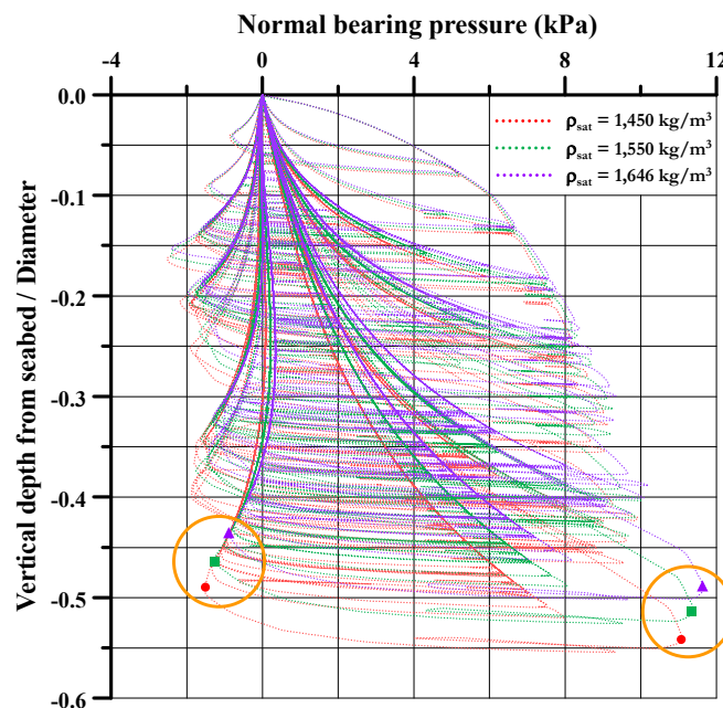
Fig. 12 Pipe embedment by saturated soil density variation.
