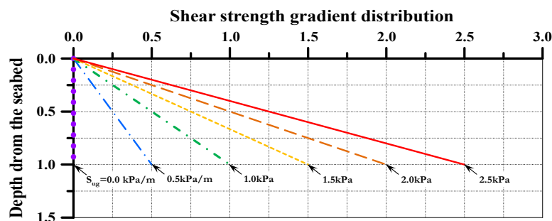
Fig. 6 Shear strength gradient distribution.
