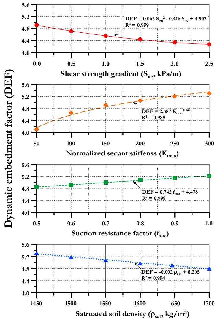
Fig. 13 Dynamic embedment factor by nonlinear soil parameters.
