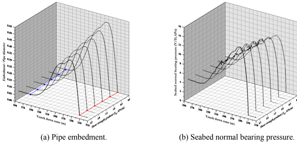
Fig. 7 Pipe embedment and normal bearing pressure by shear strength gradient variation.
