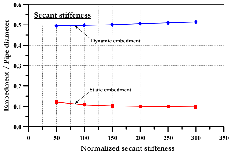
Fig. 9 Pipe embedment for normalized secant stiffness.
