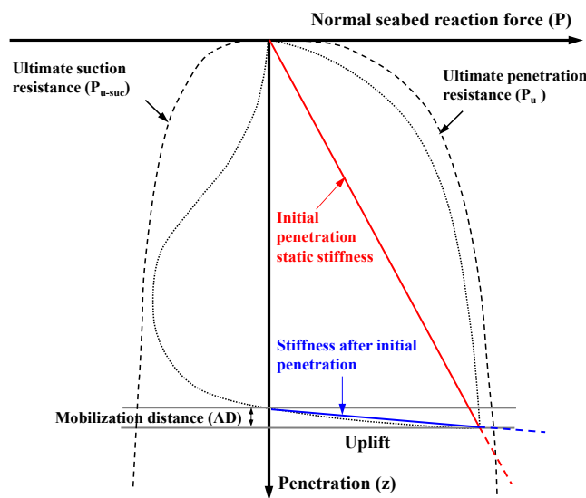
Fig. 8 Static and dynamic soil stiffness (Bridge, 2005).
