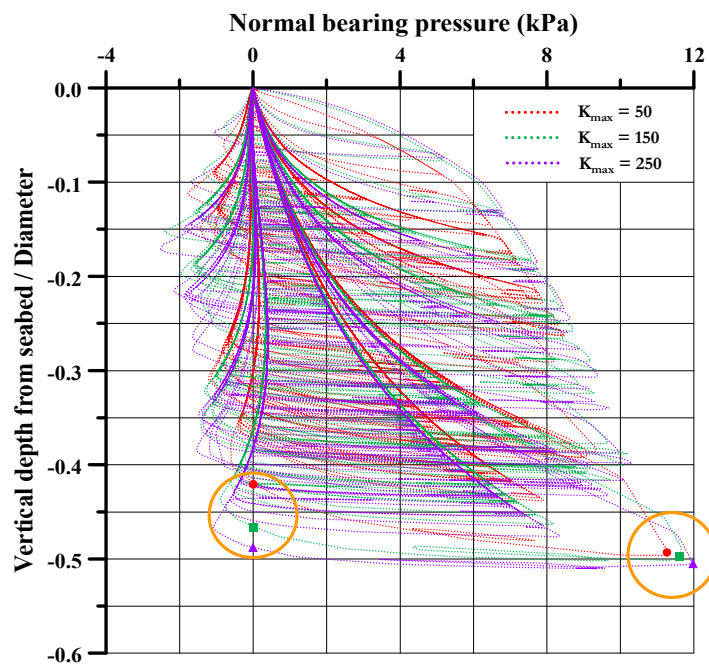
Fig. 10 Pipe embedment behavior by normalized secant stiffness.
