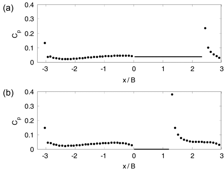
Fig. 7 Pressure coefficient distribution at 1/4-buttock line. Points, on the hull surface; solid line, inside the air cavity. (a) air-cavity hull, (b) stepped planing hull.
