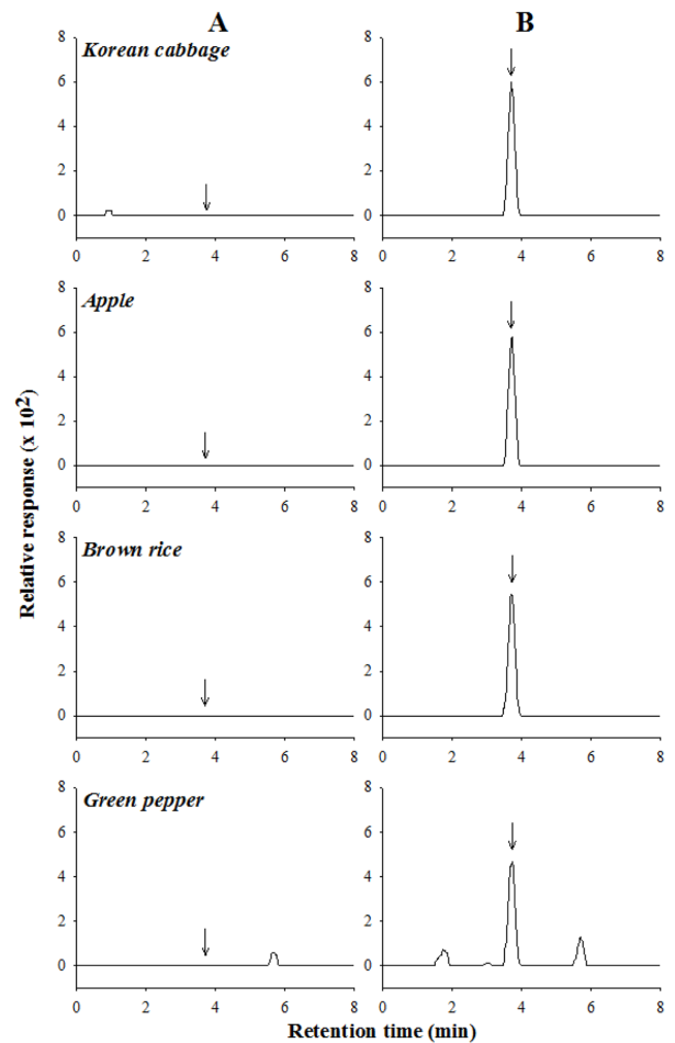
Fig. 7. LC/MS SIM chromatograms of carpropamid in crop extracts. A; control, B; fortified with carpropamid at 0.2 mg/kg.
