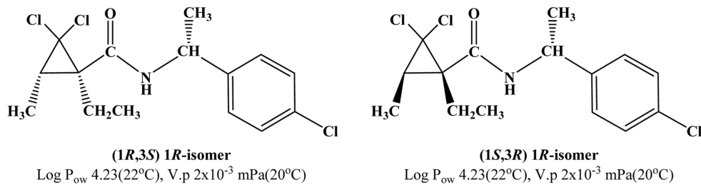
Fig. 1. Chemical structure and physico-chemical properties of carpropamid.
