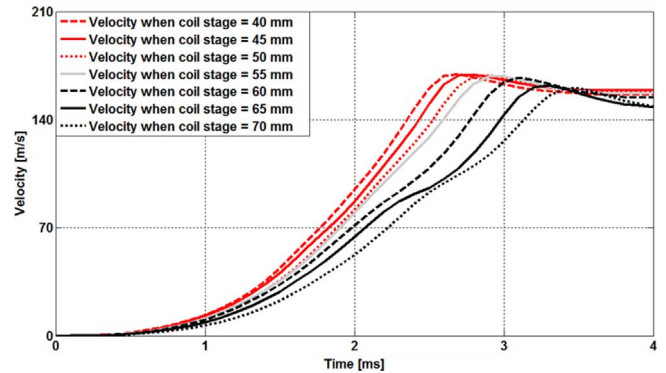
Fig. 13. (Color online) Detailed results for the velocity of the projectile for different aligned coil length in the case of an overlapped coilgun.
