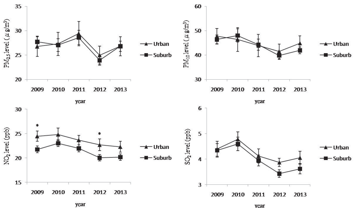
Figure 2. The air Quality Status in Northern Taiwan for the year 2009 to 2013, cited and analyzed from the Taiwan Air Quality Monitoring Network (TAQMN) of Environmental Protection Administration (EPA)
