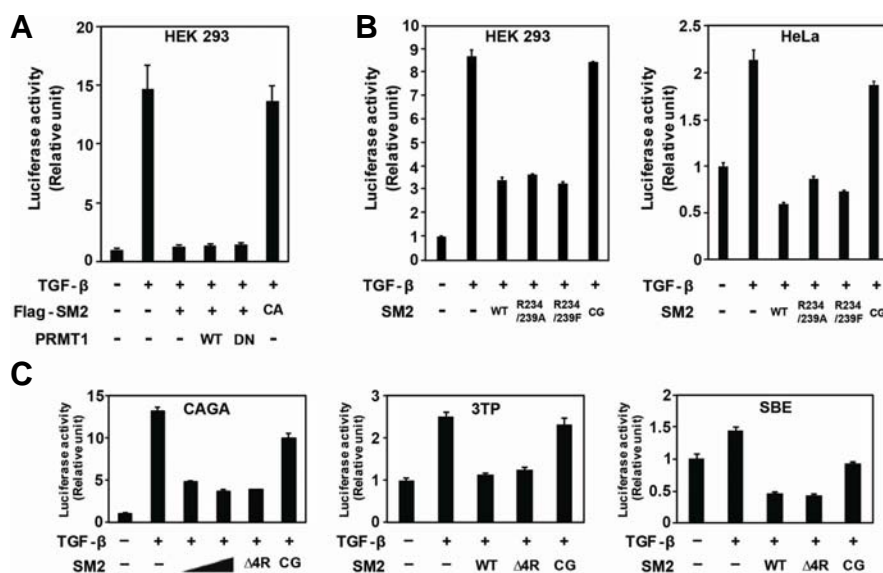
Fig. 5. PRMT1-mediated methylation has no effect on inhibitory role of Smurf2 in TGF-β signaling. (A-C) TGF-β signaling was measured based on Smad3/4-specific CAGA12-luciferase activity (A, B). pCAGA12-luc, 3TP-luc, or SBE-luc construct was co-transfected with thymidine kinase promoter-driven Renilla luciferase (pRL-TK) and indicated plasmids (C). TGF-β was treated overnight, and relative luciferase activity was measured. CG; catalytic inactive form, R234/239A; non-methylation mimetic form, R234/239F; methylation mimetic form, Δ4R; deletion of seven amino acids, including four arginines. Data represent average values from one representative experiment performed in triplicate. Error bars indicate standard deviations of triplicate.
