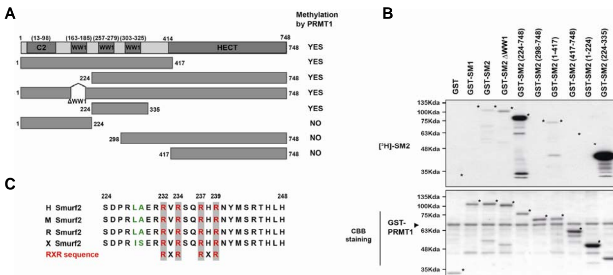
Fig. 3. Mapping of methylation domains of Smurf2 by PRMT1. (A) Schematic diagram of deletion constructs of Smurf2 and methylation results are summarized on the right side. (B) In vitro methylation assay. Purified GST fusion proteins indicated in Fig. 3A were incubated with PRMT1 in the presence of [ 3 H] adenosylmethionine (SAM). Reaction products were analyzed by SDS-PAGE, followed by fluorography. Arrowheads indicate GST-PRMT1, and asterisks indicate GST, GST-Smurf1 (SM1), and various GST-Smurf2 (SM2) deletion constructs. (C) Conservation of putative methylation sites of human (H), mouse (M), rat (R), and Xenopus (X) Smurf2. Arg232, Arg234, Arg237, and Arg239 of Smurf2 are highly conserved among all Smurf2 proteins. Two amino acids of Xenopus , marked with green color, are different from others.
