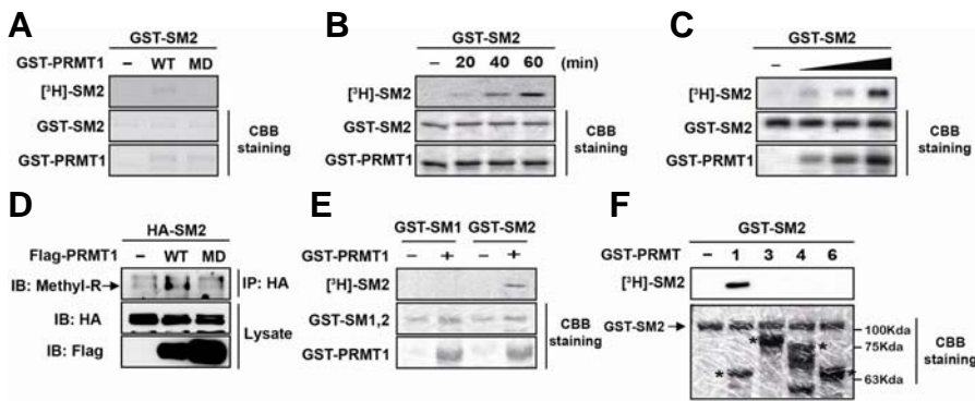
Fig. 1. Methylation of Smurf2 by PRMT1. (A) In vitro methylation assays. Purified GST-Smurf2 (SM2) was incubated with purified wild-type (WT) or methylation-dead (MD) GST-PRMT1 in the presence of [methyl- 3 H] adenosylmethionine (SAM). Reaction products were analyzed by SDS-PAGE, followed by fluorography (upper panel). Total amounts of GST-Smurf2 and GST-PRMT1 were determined by Coomassie brilliant blue (CBB) staining. (B, C) In vitro methylation of Smurf2 in a time-dependent
