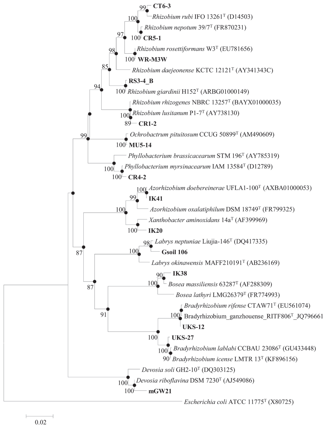
Fig. 2. Neighbor-joining phylogenetic tree, based on 16S rRNA gene sequences, showing the relationship between the strains isolated in this study and their relatives of the order Rhizobiales in the class Alphaproteobacteria . Bootstrap values (>70%) are shown above nodes for the neighbor-joining and below nodes for the maximum-likelihood methods. Filled circles indicate the nodes recovered by the two treeing methods. Bar, 0.02 substitutions per nucleotide position.
