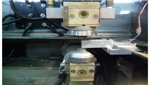
Fig. 2 Experimental setup for the hybrid WEDM
