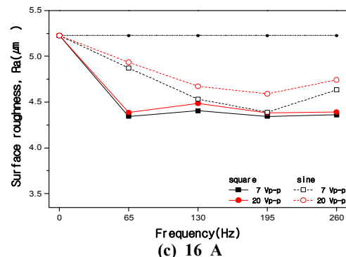
Fig. 6 Surface roughness according to frequency of vertical vibration
