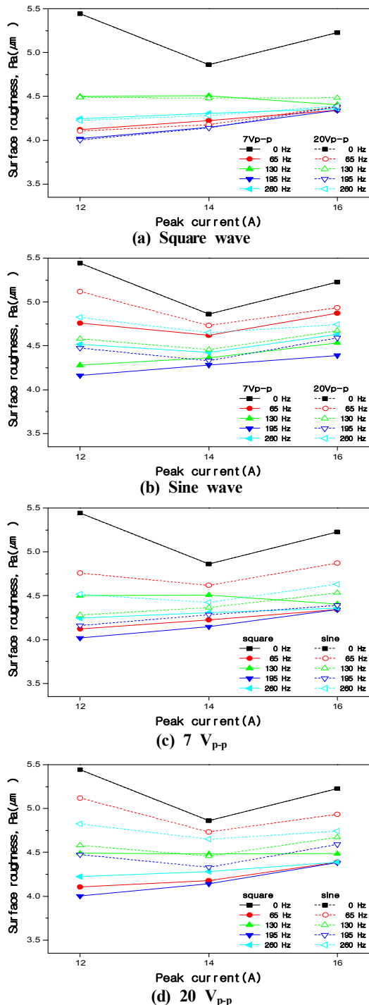
Fig. 5 Surface roughness according to peak current of vertical vibration
