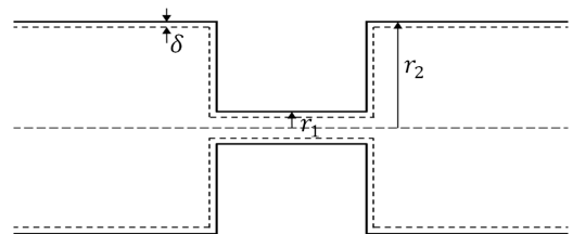
Fig. 3. Schematic view of a 'slit' sequence representing interconnected pores
