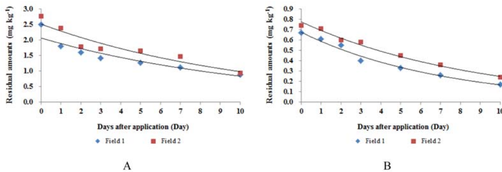
Fig. 5. Dissipation curves of pyrimethanil (A) and methoxyfenozide (B) in grape during cultivation period.
