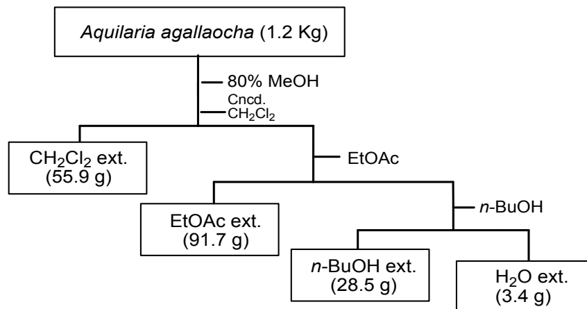
Fig. 1. Liquid-liquid partition of Aquilaria agallocha .
