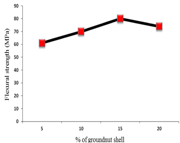
Fig. 3. Effects of variation of weight fraction on the flexural strength of groundnut shell/polyester composite
