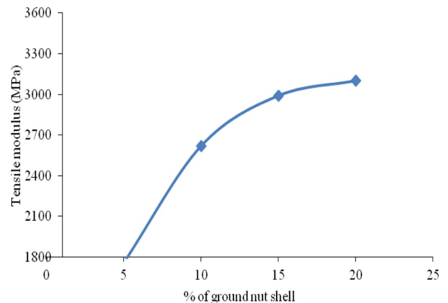
Fig. 2. Effects of variation of weight fraction on the tensile modulus of groundnut shell/polyester composite
