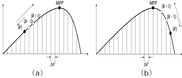
Fig. 8. Improved displacement of operating point
