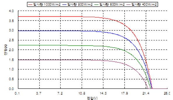
Fig. 4. I-V characteristic curve with radiation changing
