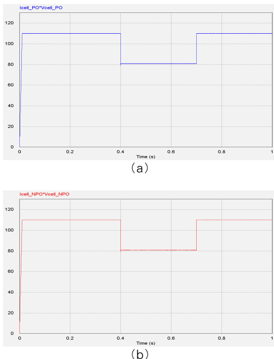
Fig. 11. Output power comparison with radiation changing
