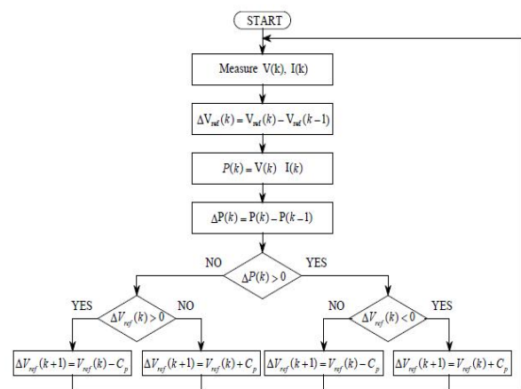
Fig. 6. MPPT control algorithm of conventional PO method
