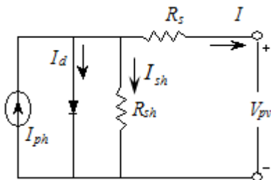
Fig. 1. Equivalent circuit of solar cell
