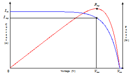
Fig. 3. I-V and P-V characteristics waveform of a solar cell
