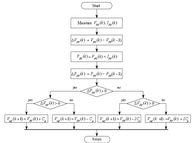
Fig. 9. Improved control algorithm of PO method
