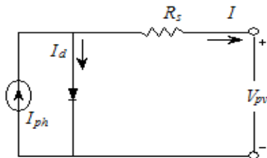
Fig. 2. Ideal Equivalent circuit of solar cell
