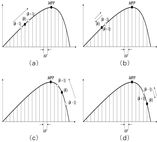
Fig. 7. displacement of operating point
