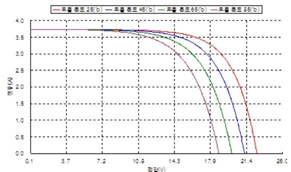
Fig. 5. I-V characteristic curve with temperature changing
