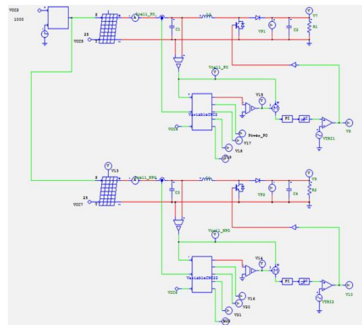
Fig. 10. PSIM circuit for MPPT control
