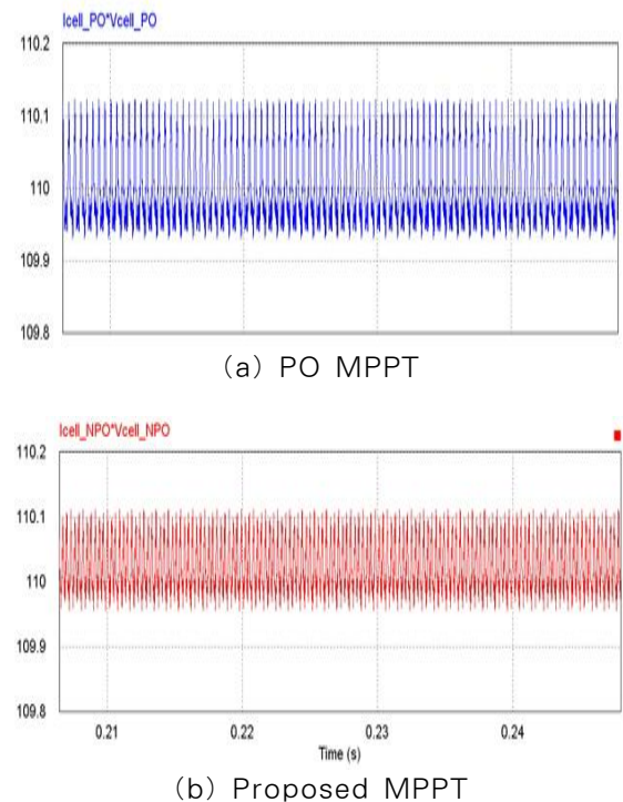
Fig. 13. Comparison of error in steady-state
