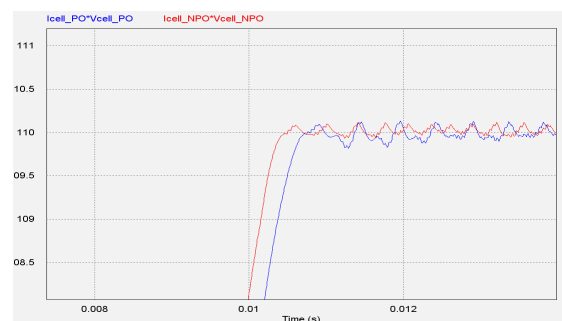
Fig. 12. Comparison of tracking speed
