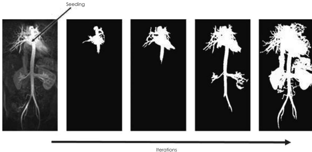
Fig. 7. Region growing.
