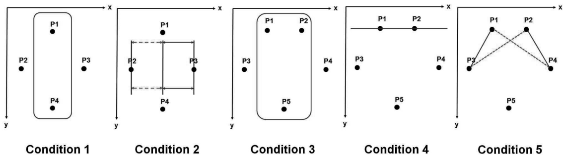
Fig. 8. Detecting conditions.
