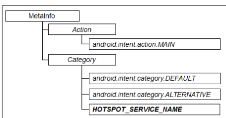
Fig. 8. MetaInfo Structure
