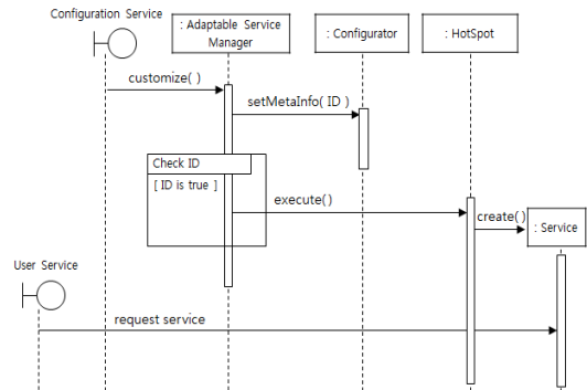
Fig. 14. Dynamic Model for Adaptable Smartwork Service
