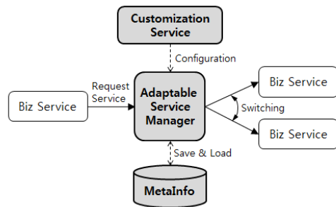
Fig. 10. Dynamic Service Architecture by Selection
