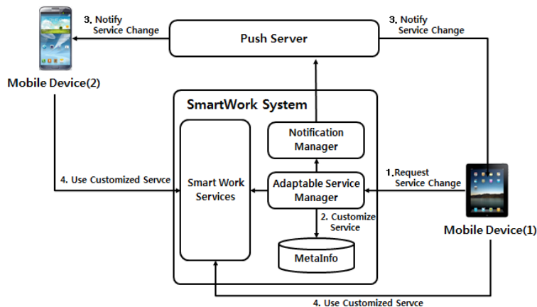
Fig. 12. Adaptable Smartwork Process
