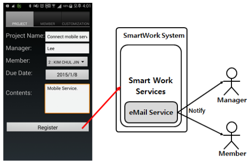
Fig. 15. SmartWork Service using eMail
