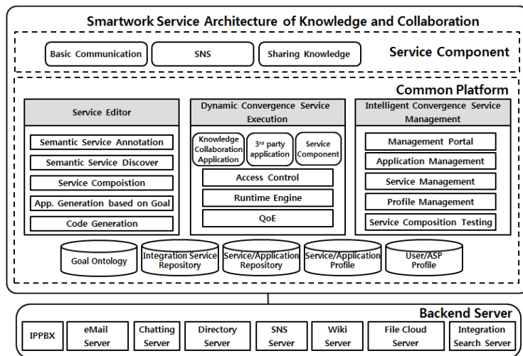
Fig. 2. Smartwork System Architecture
