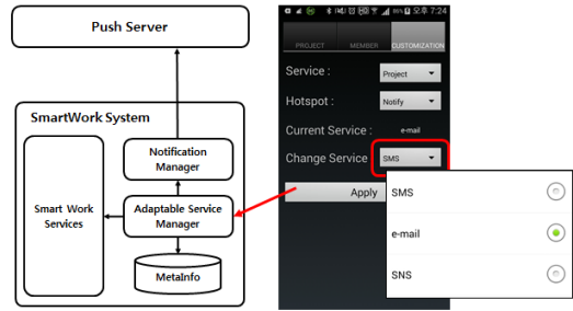
Fig. 16. Customization using Adaptable Service
