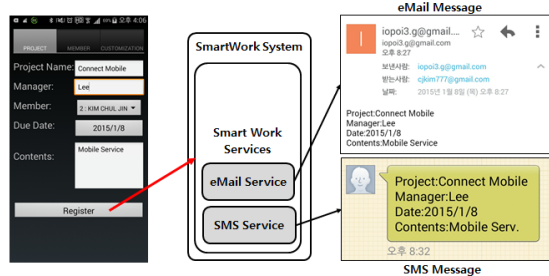
Fig. 17. Customized Service by Adaptable Service
