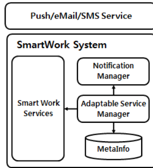
Fig. 4. Adaptable Architecture for Smartwork System
