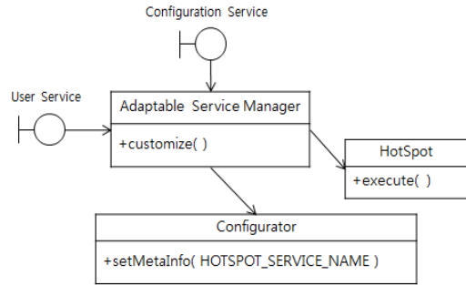
Fig. 13. Static Model for Adaptable Smartwork Service
