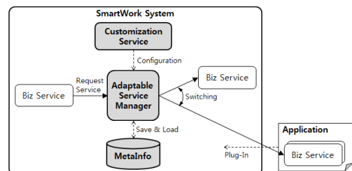
Fig. 11. Dynamic Service Architecture by PlugIn
