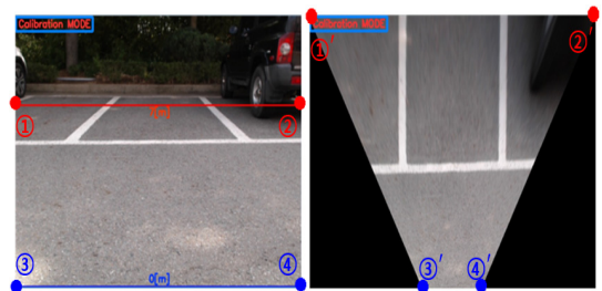
Fig. 19. Warping course
