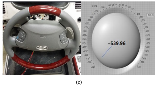
Fig. 8. Handle angle value according to the CAN signal of SAS (a)When the handle is rotated 180 degree to the right (b)When the handle is rotated 360 degree to the right (c)When the handle is rotated 540 degree to the left
