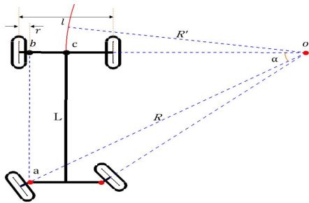
Fig. 2. Turning radian when vehicle reversing
