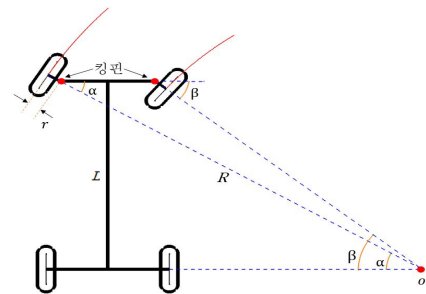
Fig. 1. Minimum turning radius when vehicle turning
