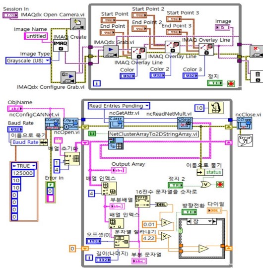
Fig. 7. LabVIEW block diagram
