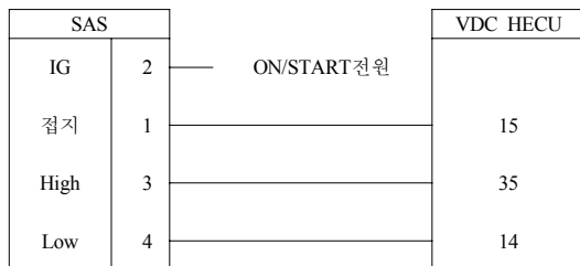
Fig. 4. Circuit diagram of SAS
