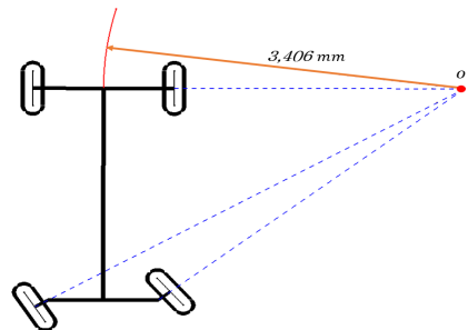
Fig. 3. Turning radian when the handle steering is 540 degree
