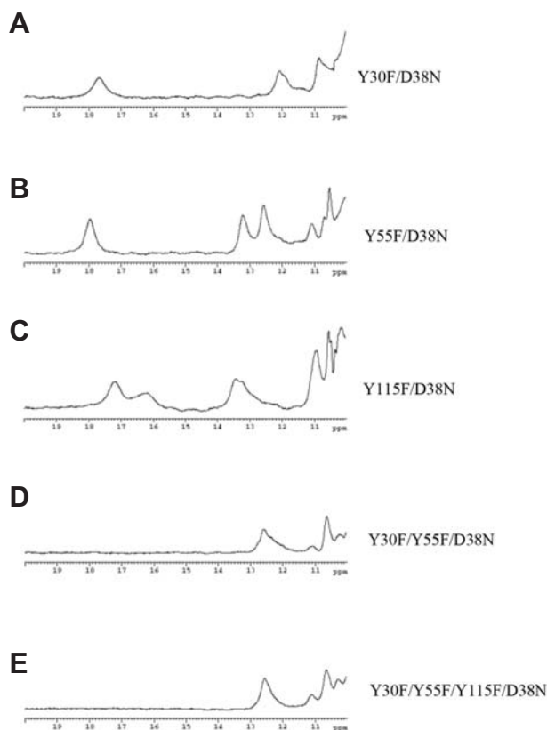
Fig. 2. 1 H NMR spectra of P. putida KSIs. (A) Y30F/D38N at pH 8.5, (B) Y55F/D38N at pH 7.0, (C) Y115F/D38N at pH 8.5, (D) Y30F/Y55F/D38N at pH 8.5, (E) Y30F/Y55F/Y115F/D38N at pH 7.0, which are complexed with equilenin, respectively. The concentration of KSI is 10 mg/ml and the concentration of DMSO- d_6 10%.
