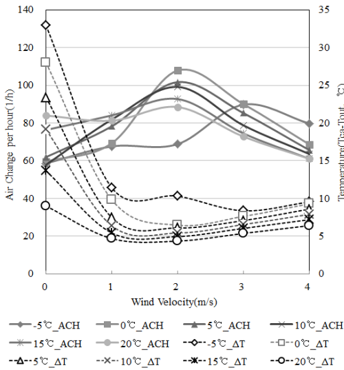
Fig. 7. Result of Case 2_150W/m 2 (Wind and Buoyancy Effect)
