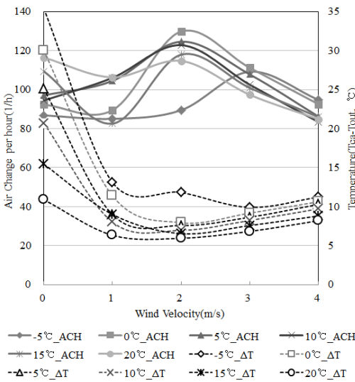
Fig. 8. Result of Case 2_250W/m 2 (Wind and Buoyancy Effect)
