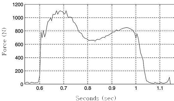
Fig. 1. Footfall force of a 870N male at 2.4Hz (Brownjohn, 2006)
