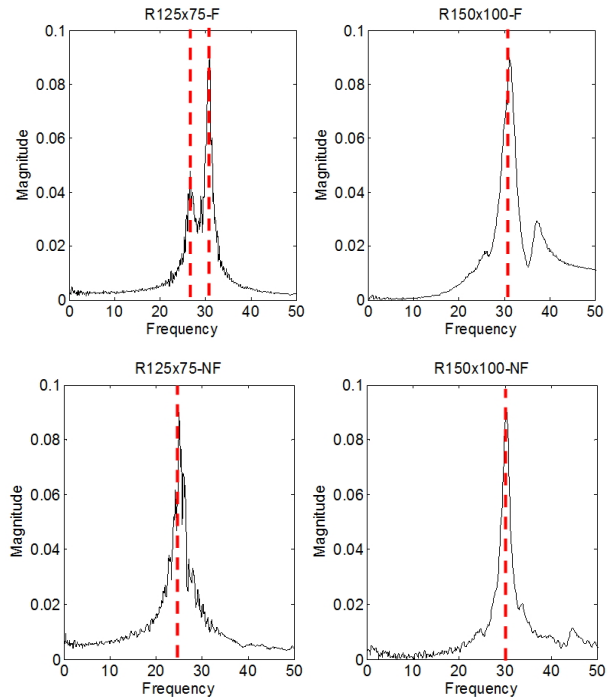
Fig. 4. Frequency response (clockwise from top left) R-□125x75x4.5-F, R-□150x100x4.5-F, R-□150x100x4.5-NF and R-□125x75x4.5-NF
