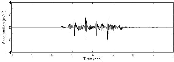
(b) Walking on fast pace (3.4Hz walking frequency)
