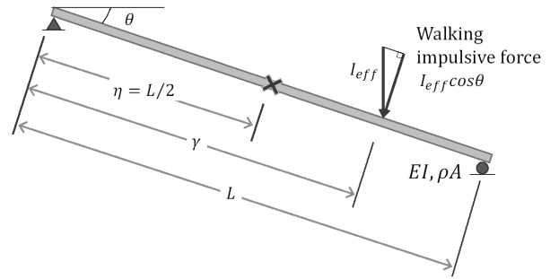
Fig. 7. Applied walking impulsive force and key symbols
