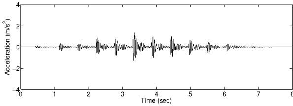
(a) Walking on normal pace (1.8Hz walking frequency)
