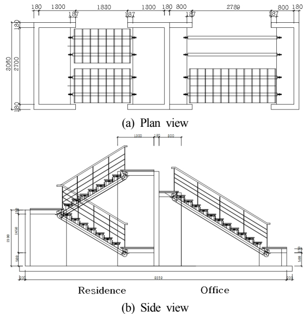
Fig. 3. Schematic drawings for test specimen
