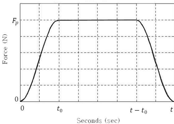
Fig. 2. Idealized footfall force (Brownjohn, 2006)
