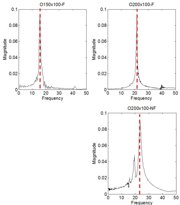
Fig. 5. Frequency response (clockwise from top left) O-□150x100x4.5-F, O-□200x100x4.5-F and O-□200x100x4.5-NF
