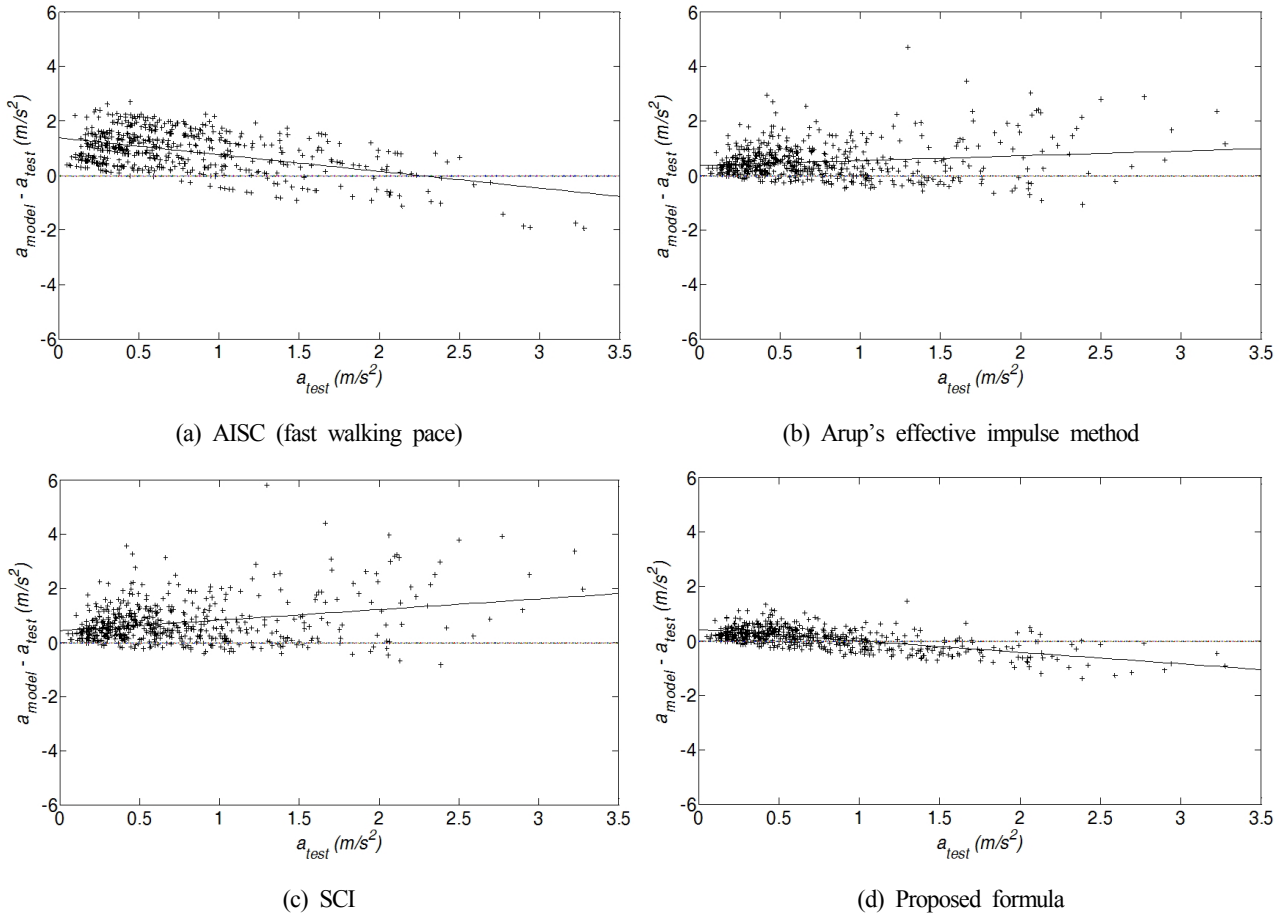
Fig. 9. Residual plots for each model
