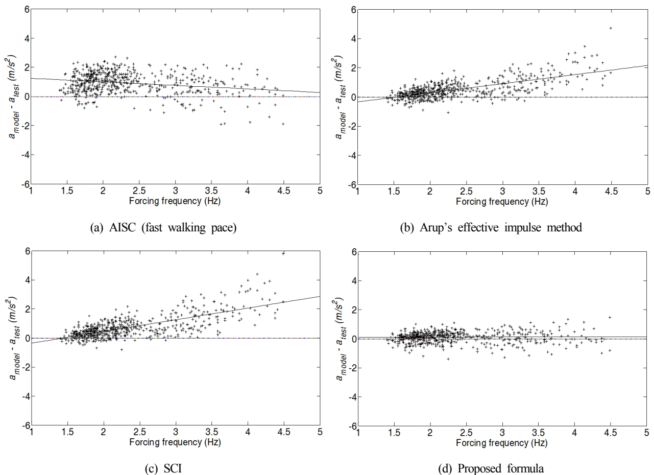
Fig. 10. Residual acceleration responses concerning with forcing frequency
