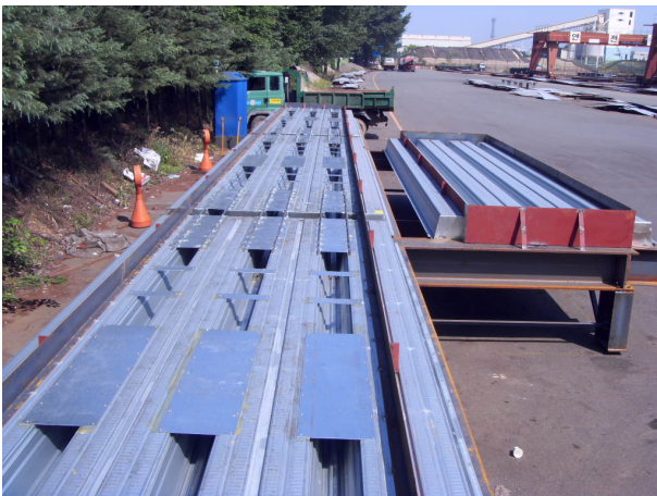
Fig. 7. preliminary specimens
