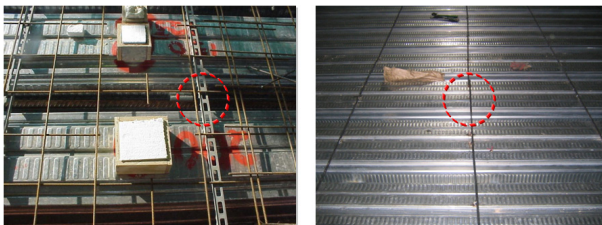
Fig. 2. Prevent flaring of the upper deck
