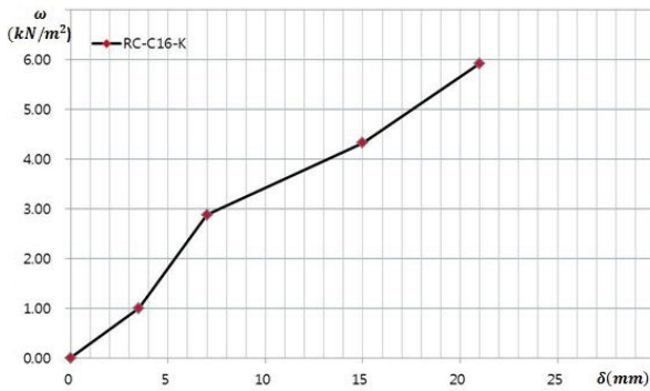
Fig. 13. Center deflection in each load step: RC-C16-K
