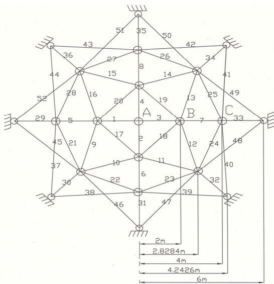
Fig. 12. Initial configuration of the 52-bar truss
