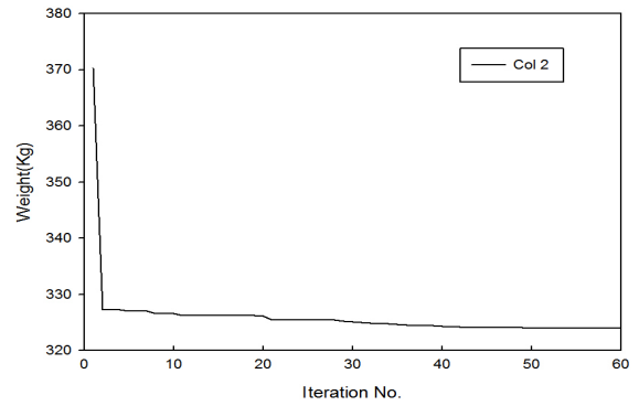
Fig. 6. Convergence behaviour of 72-bar truss
