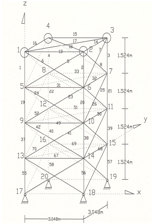
Fig. 5. 72-bar truss structure
