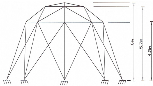
Fig. 13. Initial configuration of 52-bar truss (side view)
