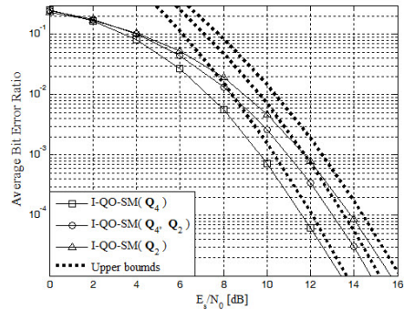
Fig. 3. BERs versus E_s/N_0 [dB] for proposed I-QO-SMs at 10 bits/channel use.
