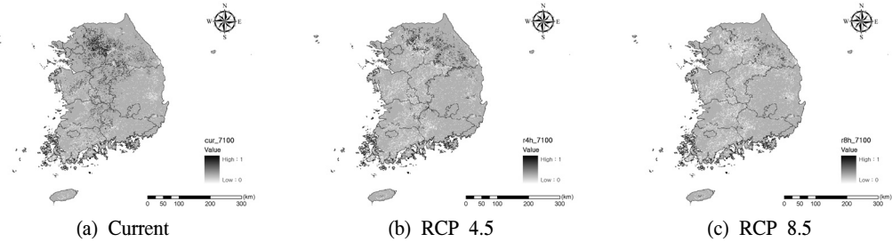
Figure 8. Current(1971~2000) and long-term future(2071~2100) of Korean pine ( Pinus koraiensis ).
