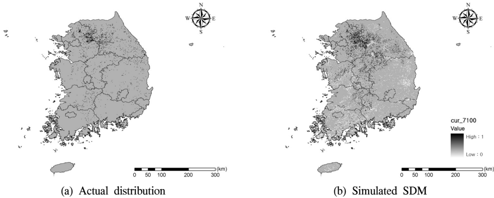
Figure 3. Actual distribution and simulated SDM of Korean pine ( Pinus koraiensis ).
