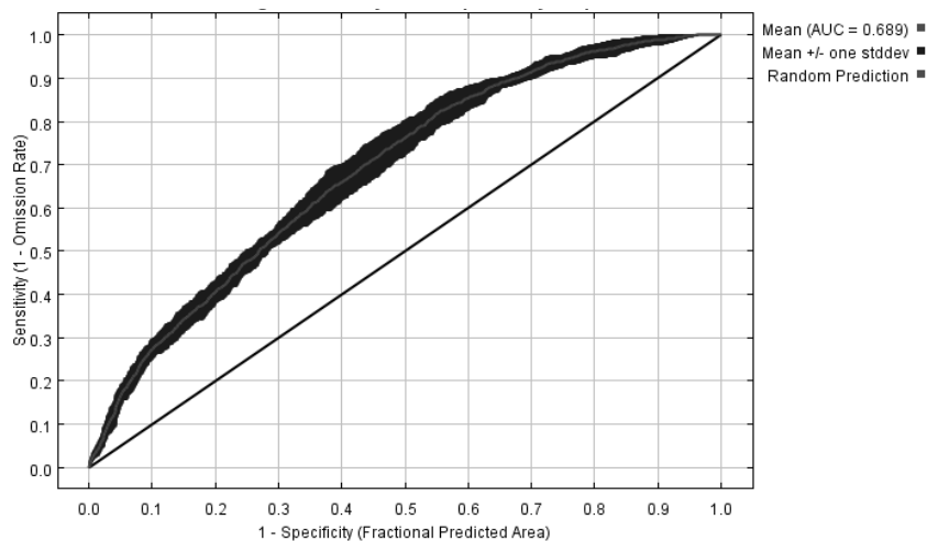
Figure 1. Average Sensitivity vs. 1 - Specificity of Korean pine ( Pinus koraiensis ).
