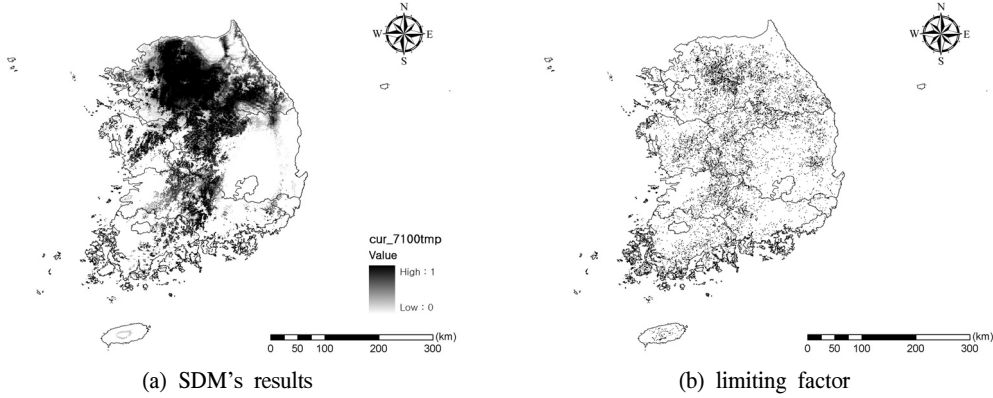
Figure 2. SDM's results and limiting factor of Korean pine ( Pinus koraiensis ).
