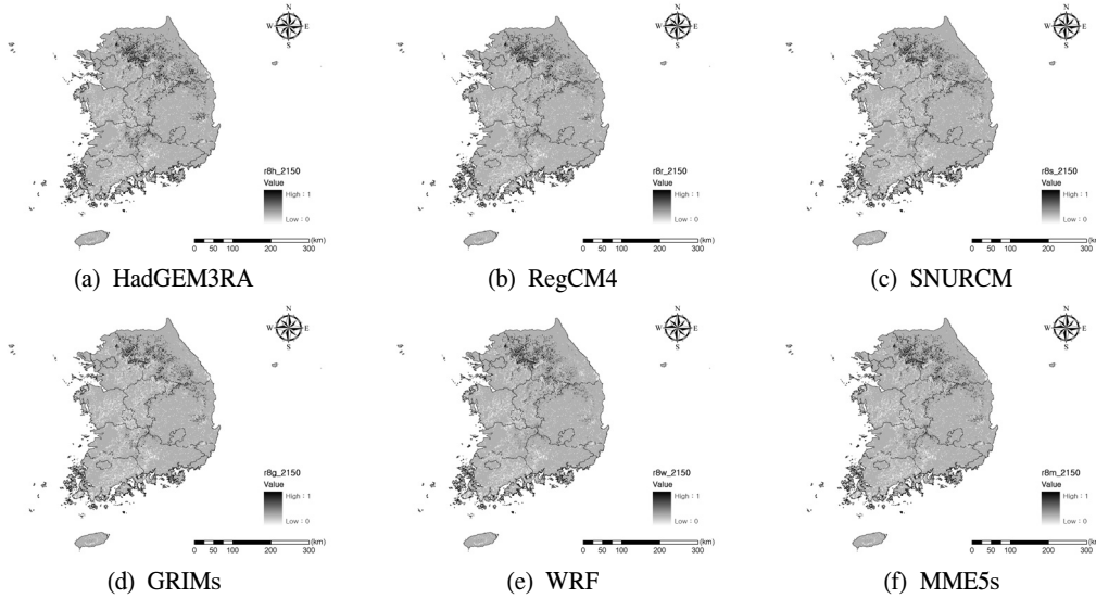
Figure 6. Distribution map of Korean pine ( Pinus koraiensis ) on RCP 8.5 Scenarios.
