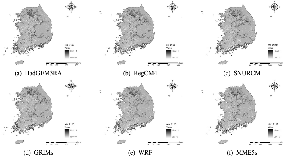
Figure 4. Distribution map of Korean pine( Pinus koraiensis ) on RCP 4.5 Scenarios.
