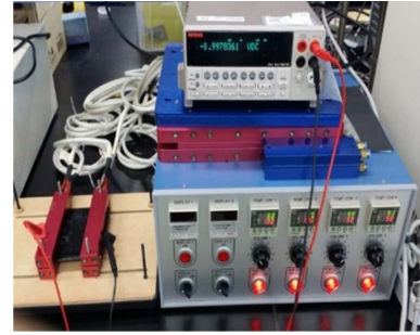
Fig. 5. Seebeck coefficient measuring setup
