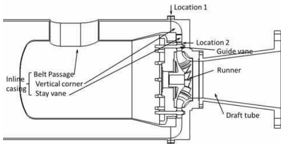
Fig. 2 Cross sectional view of turbine flow passage
