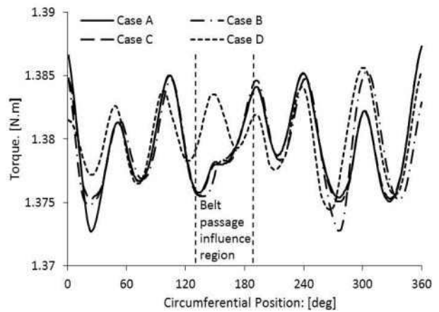
Fig. 10 Torque distribution on the runner single blade
