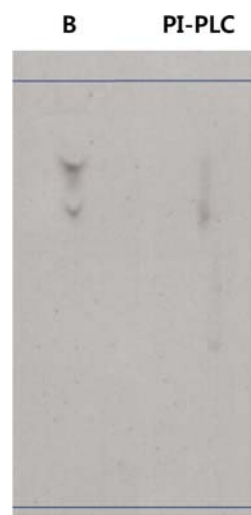
Fig. 2 Phospholipase sensitivity of glycosylphosphatidylinositol spots on TLC plates. Silica powder in the area between Rf 0.6–0.9 on the silica plate (Fig. 1) was excised with a blade and extracted with n -butanol. The extract was then reacted with buffer (B) only or PI-specific phospholipase C (PI-PLC), respectively, and developed on TLC plates. Two spots represent PI-GlcNAc (Rf = 0.76) and PI-GlcN (Rf = 0.70), respectively.
