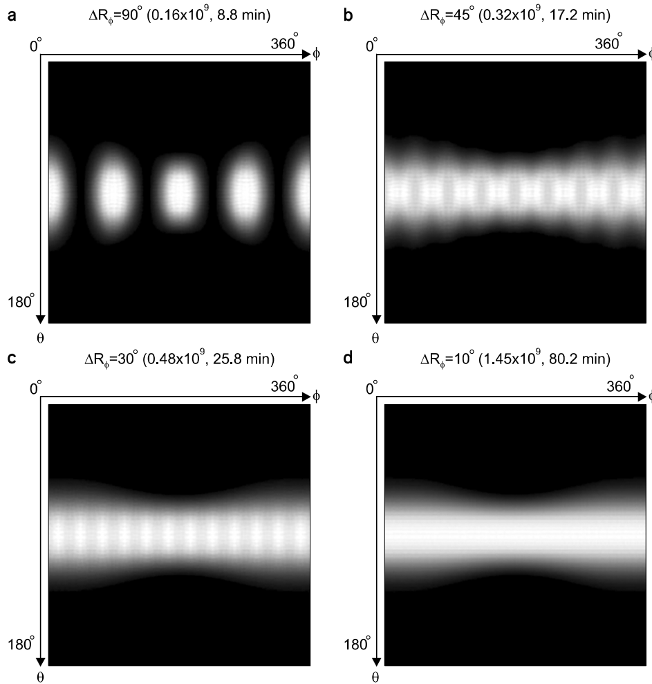
Fig. 8. Histogram of spherical angles \theta and \phi for the sampled lines on the detected conical surfaces in rotating Compton camera with (a) \Delta R_\phi=90^\circ , (b) \Delta R_\phi=45^\circ , (c) \Delta R_\phi=30^\circ , (d) \Delta R_\phi=10^\circ .
