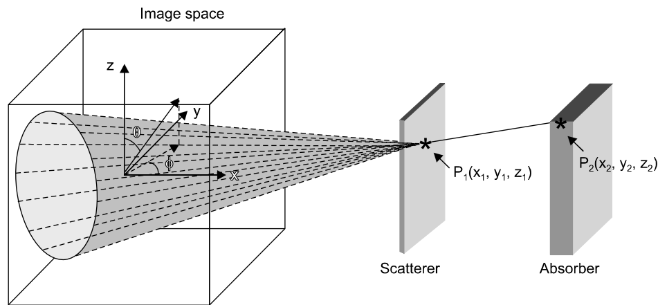
Fig. 4. Sampling technique of lines on conical surface defined with two detection positions and a scattering angle and the corresponding angles \theta and \phi of the sampled lines in spherical coordinate.
