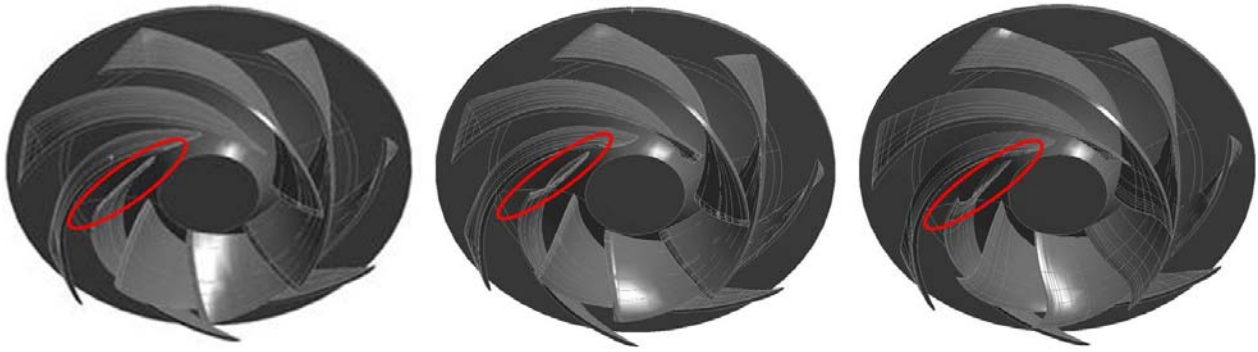
Fig. 3 3 cases with different type of blade low pressure side shape
