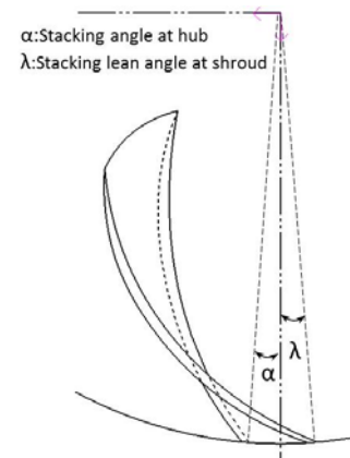
Fig. 5 Definition of stacking angle at blade high pressure side
