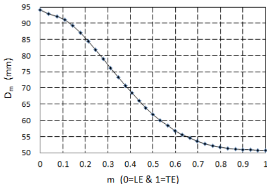
Fig. 2 Diameter distribution of the inscribed circle
