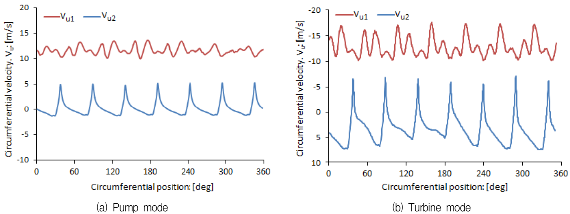
Fig. 12 Circumferential velocity distribution at impeller inlet and outlet_Normal operating: (a) pump mode; (b) turbine mode
