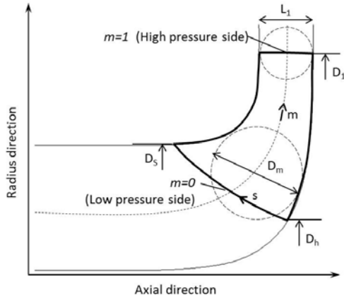
Fig. 1 Sketch of impeller meridional shape
