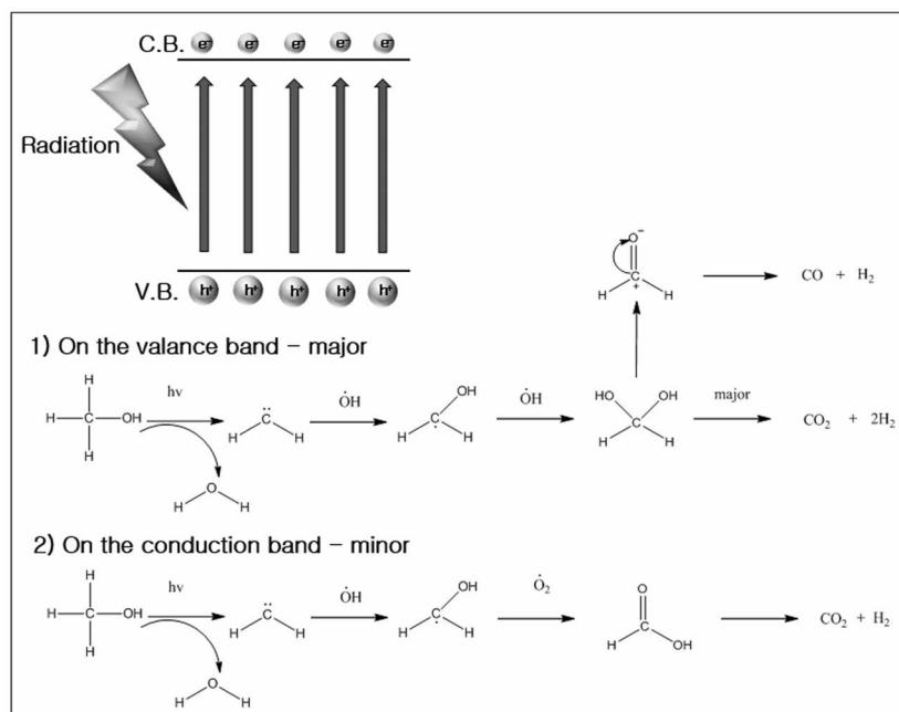
Figure 10. The expected mechanism for the production of H 2 from water/methanol photodecomposition over the Ag x O/P25-TiO 2 photocatalyst.
