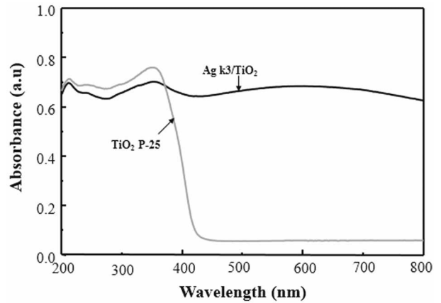
Figure 6. UV-visible diffuse reflectance spectra K3-Ag x O/P25-TiO 2 .
