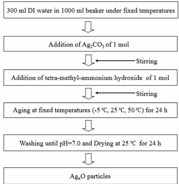
Figure 1. Preparation procedure of Ag x O particles by a conventional sol-gel method.
