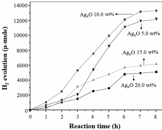
Figure 8. The H 2 productions from water/methanol photodecomposition according to the weight ratio of Ag x O (5, 10, 15, 20 wt%).
