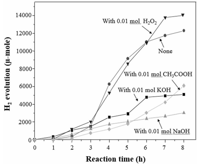
Figure 9. H 2 productions from water/methanol photodecomposition over the mixture with different additive (H 2 O 2 , NaOH, KOH, CH 3 COOH).
