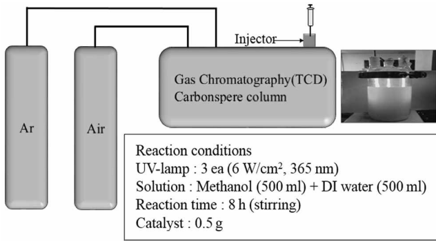
Figure 2. Batch-type liquid photo system.
