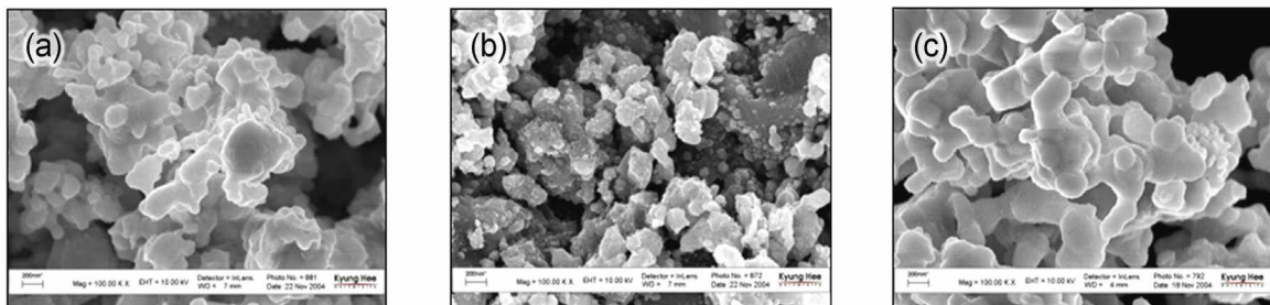
Figure 4. SEM images of the Ag x O particles treated at various temperatures. a) K1 = -5 °C Ag x O, b) K2 = 25 °C Ag x O, and c) K3 = 50 °C Ag x O.
