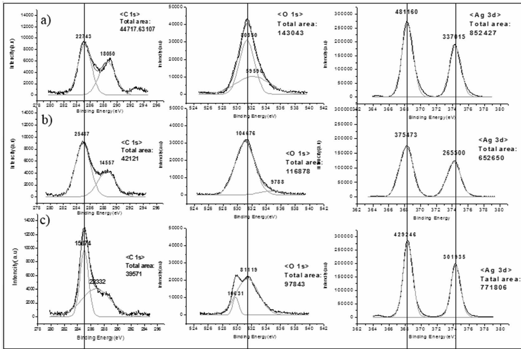
Figure 5. XPS resolutions of the Ag x O particles treated at various temperatures. a) K1 = -5 °C Ag x O, b) K2 = 25 °C Ag x O, and c) K3 = 50 °C Ag x O.
