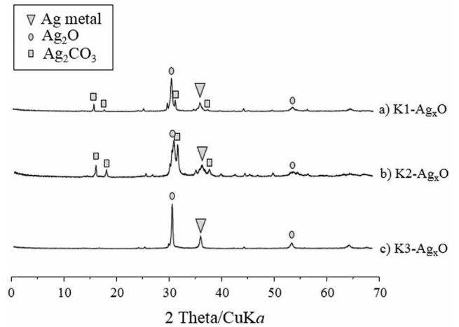
Figure 3. XRD patterns of the Ag x O particles treated at various temperatures.
