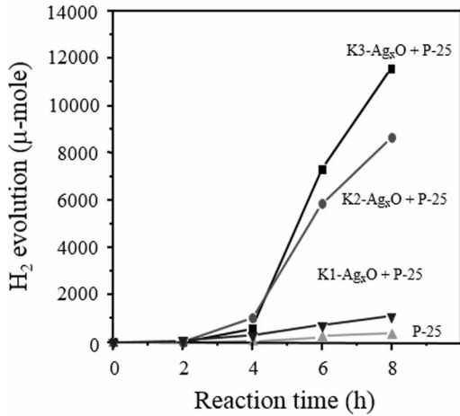
Figure 7. H 2 productions from water/methanol photodecomposition over the mixture of treated Ag x O/P25-TiO 2 photocatalysts (K1 = -5 °C, K2 = 25 °C and K3 = 50 °C).
