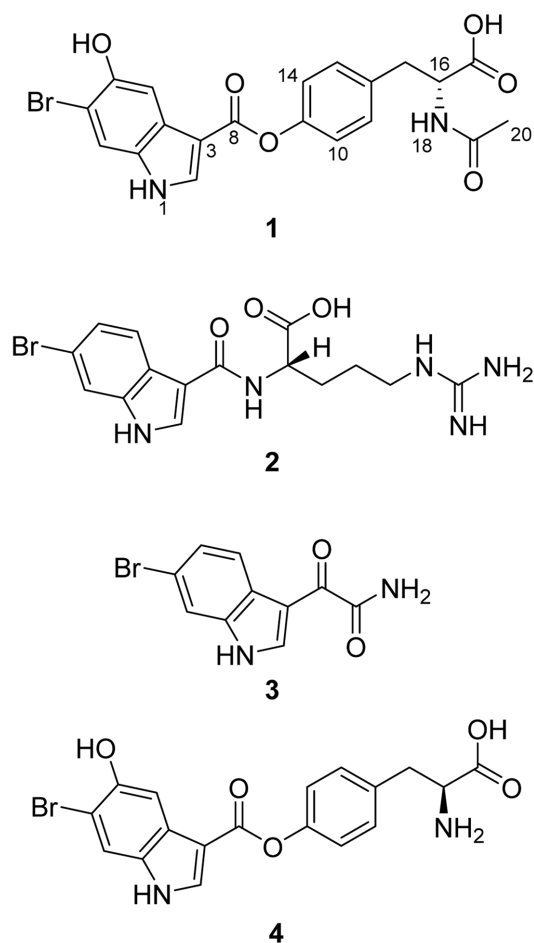
Fig. 1. Structures of compounds 1 - 3 from a marine colonial tunicate Didemnum sp. and herdmanine D (4).
