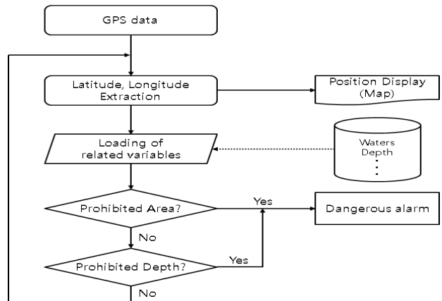
Figure 10: prohibition area warning processor
