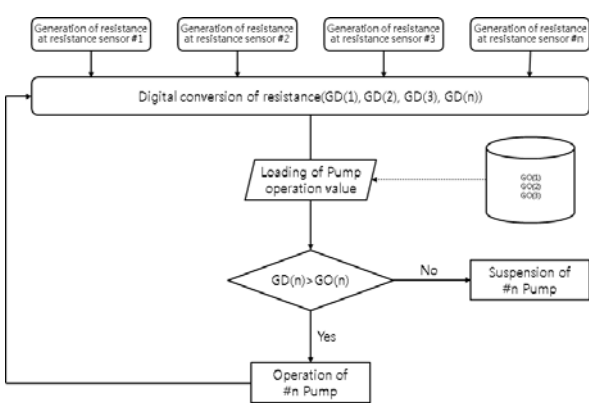
Figure 4: Bilge monitoring system operation processor
