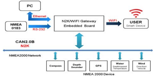
Figure 7: Architecture of N2K/WIFI gateway
