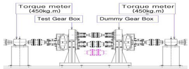
Figure 5: Details of the test jig & gear box
