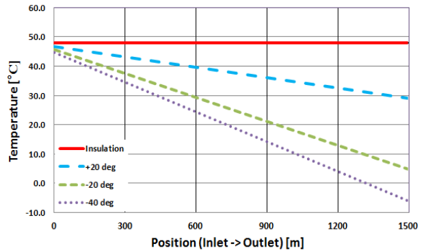
Figure 6: Temperature distribution
