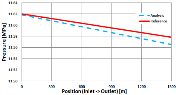
Figure 3: CFD validation
