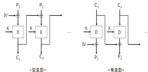
<Figure 1> CBC-Mode
