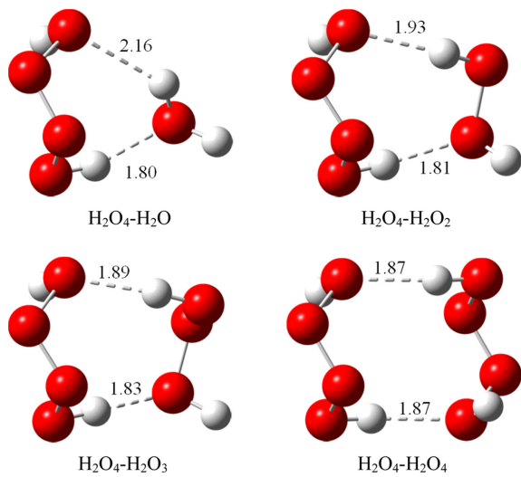
Figure 4. Optimized structures of \text{H}_2\text{O}_4\text{-H}_2\text{O}_n ( n=1-4 ) dimers at the MP2/cc-pVTZ level of theory. Bond lengths are in Å.
