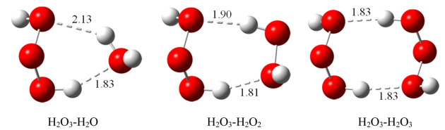
Figure 3. Optimized structures of H 2 O 3 -H 2 O n (n=1-3) dimers at the MP2/cc-pVTZ level of theory. Bond lengths are in Å.
