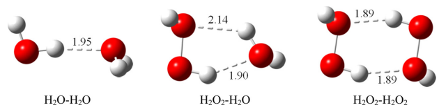
Figure 2. Optimized structures of H 2 O and H 2 O 2 dimers at the MP2/cc-pVTZ level of theory. Bond lengths are in Å.
