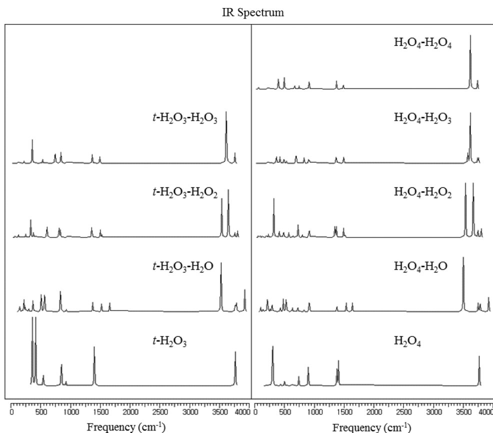
Figure 5. Predicted IR peaks for t-H 2 O 3 -H 2 O n (n=1-3) and H 2 O 4 -H 2 O m (n=1-4) at the MP2/cc-pVTZ level of theory.
