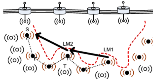
Fig. 4. Void handling mode in HydroCast [40]
