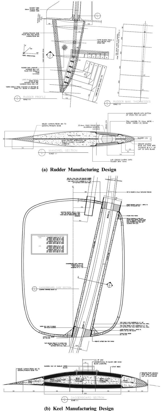
Fig. 3. Rudder/Keel Composite Manufacturing Design
