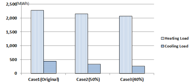
Fig. 2. Load graph(A)
