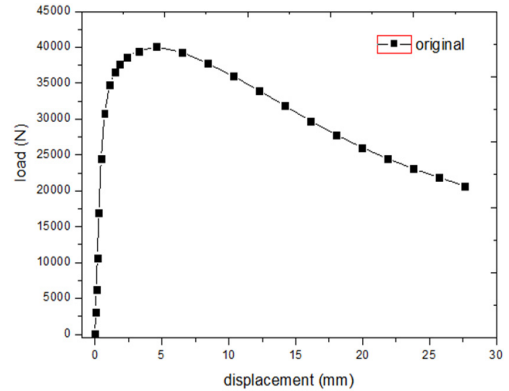
[Fig. 6] Load-Displacement Curve of AL6082 OTR.
