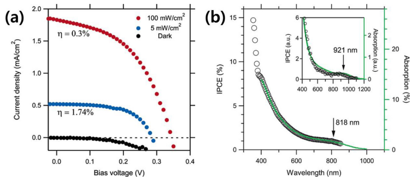
Fig. 2. (a) J-V characteristic of a QDSSC with 3.4-nm InAs QD sensitizers under different illumination intensities. (b) IPCE of a QDSSC using 3.4-nm InAs QD sensitizers while the inset IPCE from a QDSSC using 4.5-nm InAs QDs. (Reprinted with permission from ref. 14).
