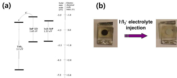
Fig. 1. (a) Schematic band diagram of InP QD/ TiO_2 interface and bulk InP (Reprinted with permission from ref. 9). (b) Photographs of PbS-sensitized solar cells before and after injection of typical I/I_3^- electrolyte.
