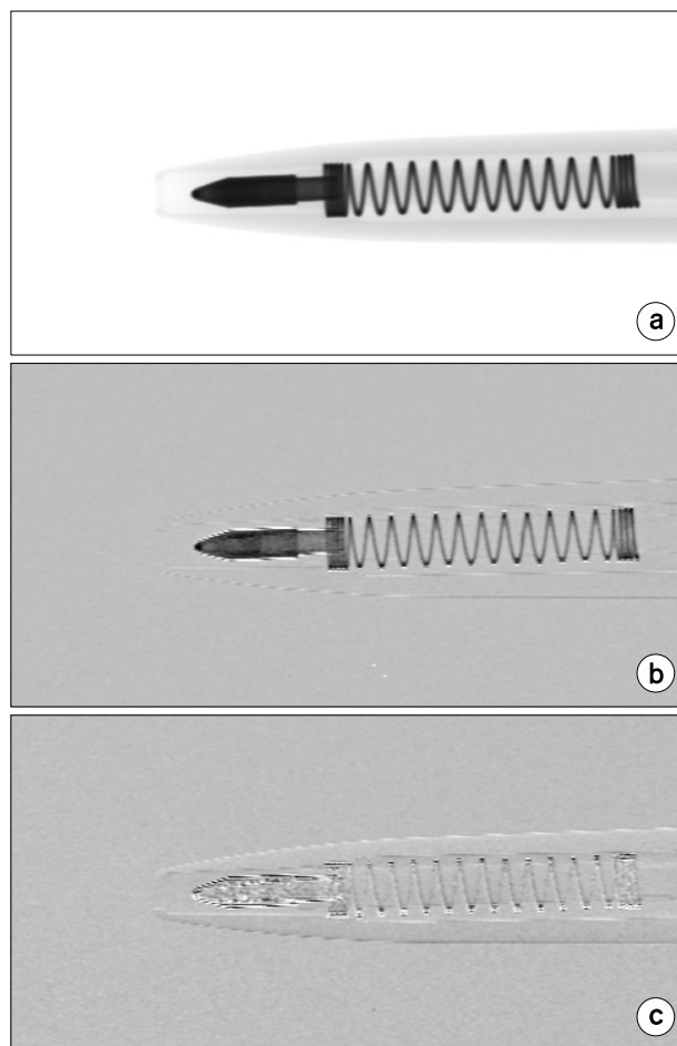
Fig. 8. Complete sets of results retrieved from a single raw image of a ball-point pen in Fig. 7 taken at x-ray tube conditions of 90\ \text{kV}_p and 0.1\ \text{mAs} : (a) the attenuation image, (b) the scattering image, and (c) the phase-contrast image.
