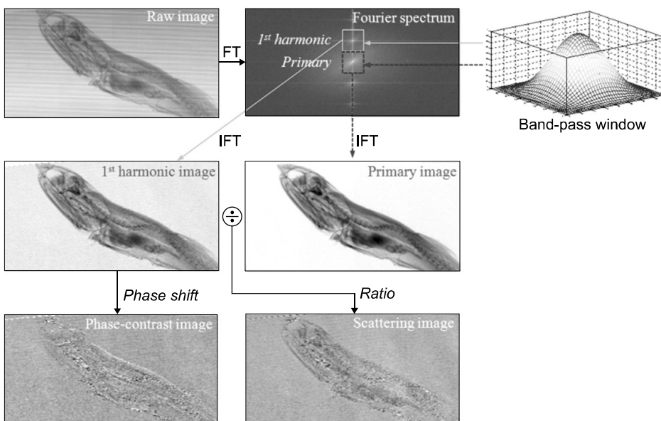
Fig. 2. Simplified single-grid-based phase-contrast x-ray imaging (PCXI) procedure. The areas surrounding the primary and the first harmonic peaks are selected separately with a band-pass filter separately, and then inverse-Fourier transformed to yield the primary image and the first harmonic image of the object.
