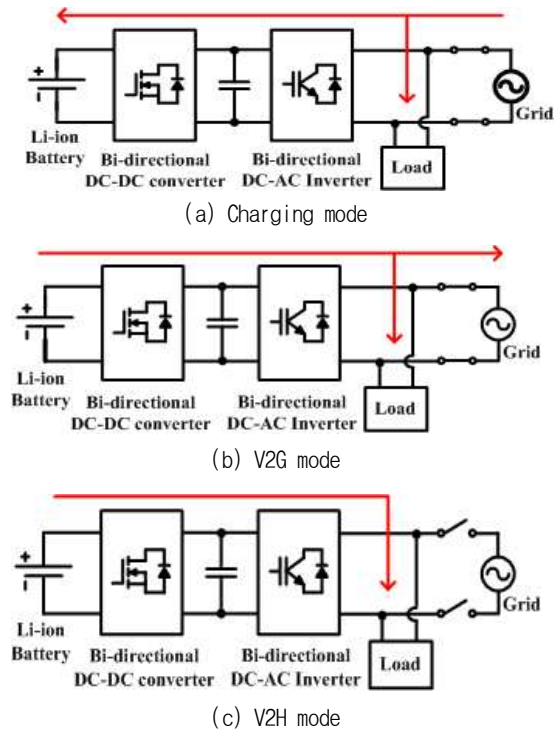
Fig. 1. Operating modes of the bi-directional battery charger.
