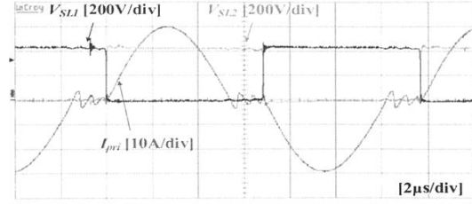
(a) Primary side of SRC
