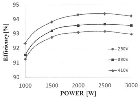
(a) Charging mode
