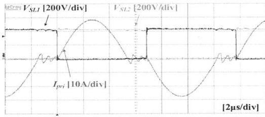
(a) Primary side of SRC
