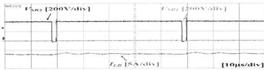
(b) Secondary side of SRC
