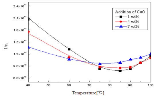
Fig. 5. The inverse of dielectric constant verse temperature of BZT-BCT ceramics with CuO addition at 1 kHz frequency (40°C ~ 100°C).
