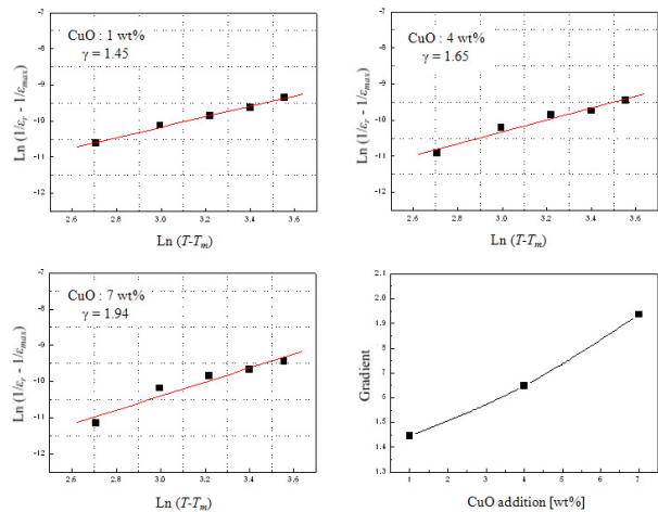
Fig. 6. Plots of \ln(1/\varepsilon_r - 1/\varepsilon_m) verse \ln(T-T_m) of BZT-BCT ceramics with CuO addition at 1 kHz frequency.
