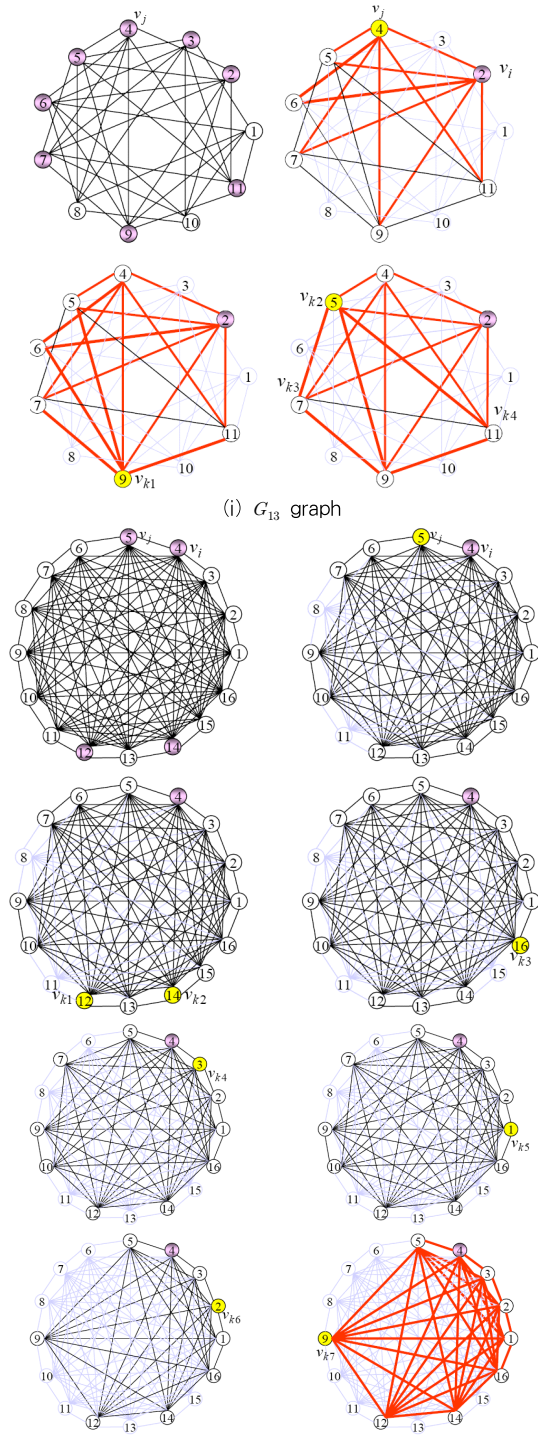
(i) G_{13} graph
