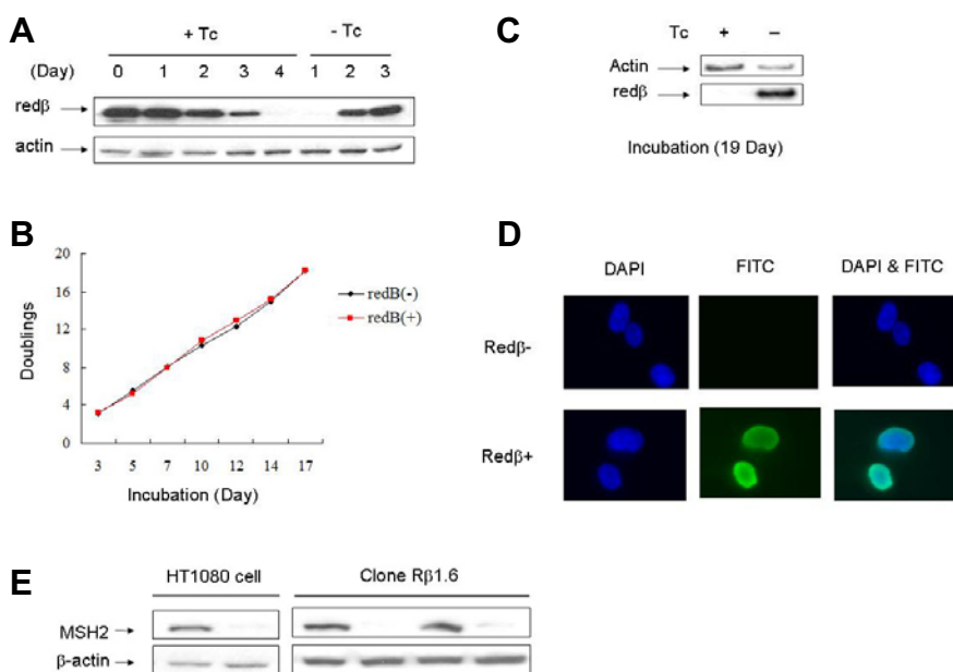
Fig. 2. Analyses of Red \beta expression and cell proliferation in clone R \beta 1.6. (A) Cells that had been grown for 4 days without tetracycline (Tet) were transferred to medium with Tet (+Tc) for 4 days and then back into medium without Tet (-Tc) for 3 days, passaging whenever necessary to avoid confluence. Samples were taken at 24 h intervals, starting at the time of Tet addition, for immunoblot analysis. (B) Measurement of doubling times for cell grown with or without Tet. (C) Immunoblot analysis of cell samples taken at day 19 from cultures analysed in (B). (D) Nuclear location of Red \beta in clone R \beta 1.6. Cells grown with (-Red \beta ) or without (+Red \beta ) Tet for > 3 days were stained with DAPI to detect DNA, and analysed for Red \beta (FITC-signal) by fluorescence microscopy. The pattern of staining shown is typical of all cells analysed. (E) MSH2 expression in siRNA-transfected cells. Immunoblot analyses of MSH2 in parental HT1080 or clone R \beta 1.6 are shown. R \beta 1.6 cells
