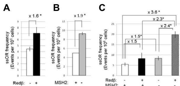
Fig. 3. Effect of Red \beta induction and MSH2 depletion on ssOR. (A) Effect of Red \beta induction on neo* correction by RO in clones R \beta 1.2, R \beta 1.6 and R \beta 1.8 (each clone assayed once). (B) Effect of MSH2 depletion on neo* gene correction by RO in HT1080 cells with or without the induction of Red \beta (n = 3). (C) The effects of Red \beta induction and MSH2 depletion, separately and together, on neo* gene correction by RO in clone R \beta 1.6. For all experiments: repair frequencies were calculated from frequencies of G418 colonies as described in “Materials and Methods”; parallel control experiments using CO in place of RO generated no G418-resistant colonies; means and standard deviations of ssO frequencies are shown for three independent experiments; numerical fold increases and significance (* indicates p-values of < 0.05; Student’ t-test) are shown.
