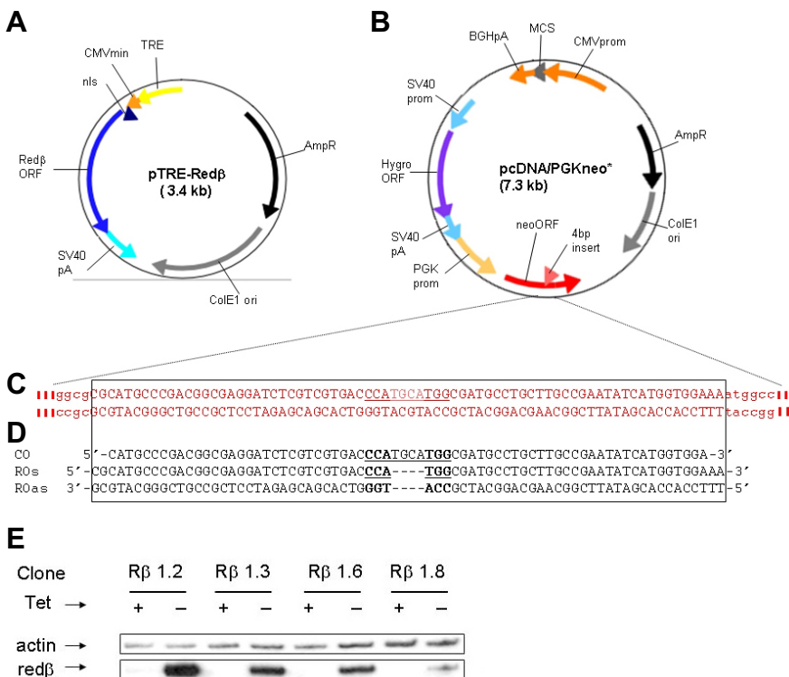
Fig. 1. Reagents used for Redβ expression and ssOR assays. (A) Structure of Redβ expression plasmid. (B) Structure of plasmid carrying the neo* target for gene correction. (C) Sequence surrounding the 4 bp insertion (bold underlined) in neo* . (D) Sequence of control (CO) and repair (RO) ssOs used in ssOR assays. (E) Immunoblot analysis of Redβ expression in hygro R clones isolated after co-transfection of HT1080 cells with the plasmids shown in (A) and (B). Clones were expanded and grown continually with tetracycline (Tet) in the growth medium (+), or for 3 days after the removal of tetracycline (-), before analysis.
