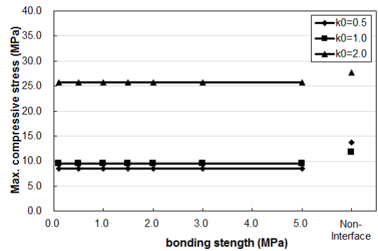
(b) Compressive stress
